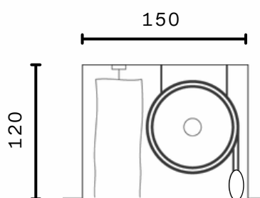
Type: P5 1 x roller & pencil/ inverted pleat curtain
