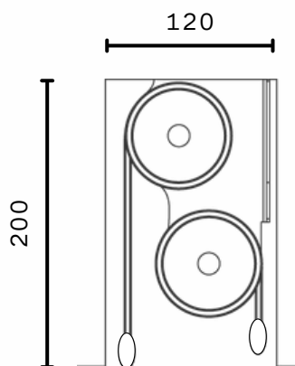
Type: P1 Dual roller reverse roll
